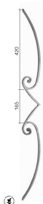
Art. GD15/3 \square 14 x 8 mm L 95 mm H 1000 mm
