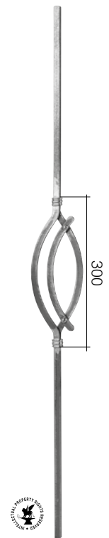
Art. GD20/7 \square 12 \text{ mm} H 1000 mm L 100 mm
