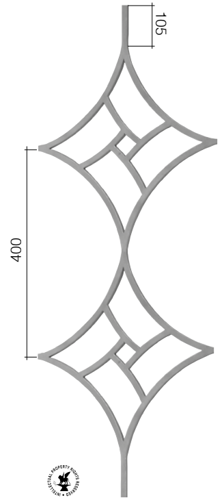
Art. GD211/4 \varnothing 12 mm L 395 mm H 1000 mm
