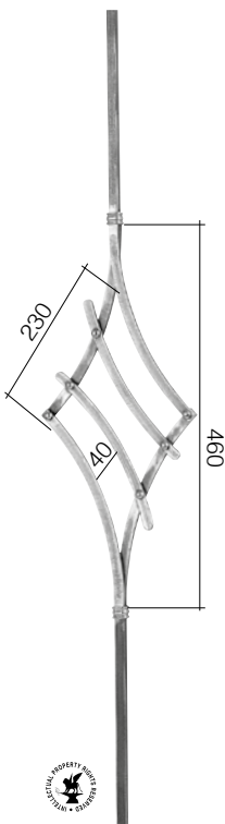
Art. GD20/8 \square 12 \text{ mm} H 1000 mm L 200 mm
