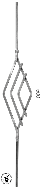
Art. GD20/3 \square 12 \text{ mm} H 1000 mm L 180 mm
