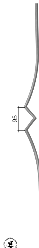
Art. GD17/1 \square 14 x 8 mm L 65 mm H 1000 mm
