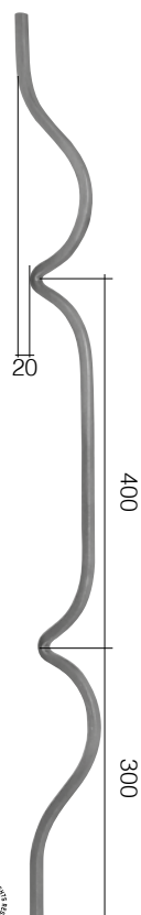
Art. GD68/3 Ø 12 mm L 105 mm H 1000 mm
