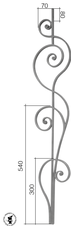
Art. GD228/2 □ 14 x 8 mm L 190 mm H 1000 mm
