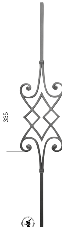
Art. GD154/3 □ 14 mm L 190 mm H 1000 mm
