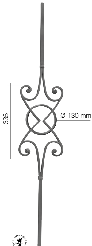
Art. GD154/2 □ 14 mm L 190 mm H 1000 mm
