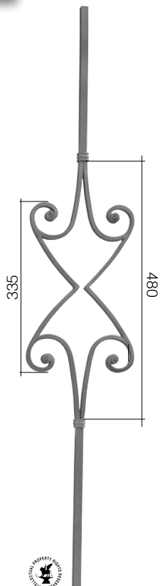
Art. GD154/1 □ 14 mm L 190 mm H 1000 mm
