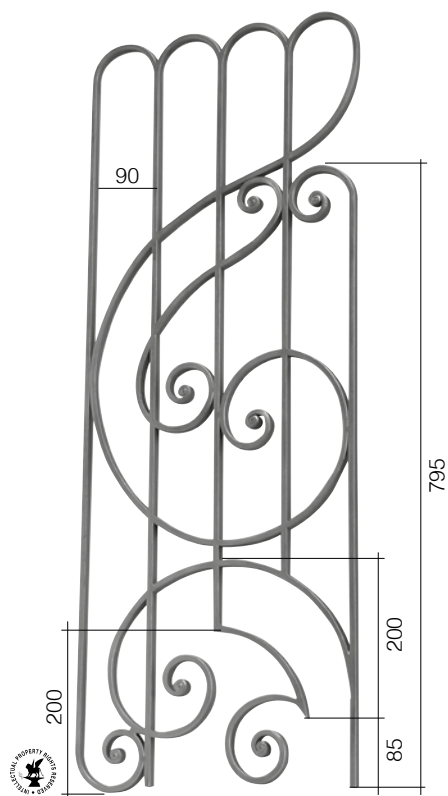
Art. GD225/1 □ 14 x 8 mm L 385 mm H 1000 mm
