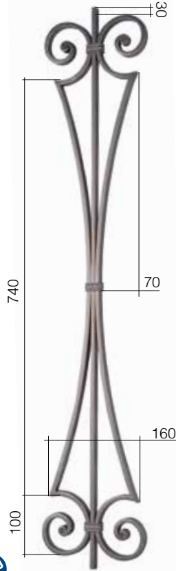
Art. GD280/1 14 x 8 mm L 200 mm H 1000 mm
