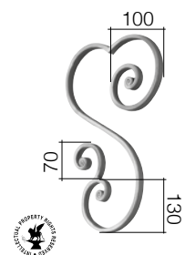
Art. GD240/2 □ 14 x 8 mm L 200 mm H 320 mm
