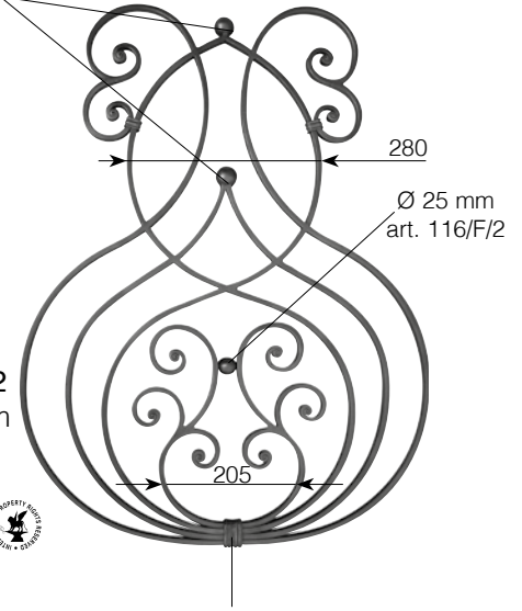
Art. GD231/2 □ 14 x 8 mm L 600 mm H 800 mm
