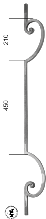
Art. GD22/2 ∅ 14 mm L 110 mm H 1000 mm
