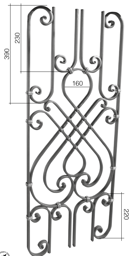
Art. GD99/1 □ 16 x 8 mm L 420 mm H 1000 mm
