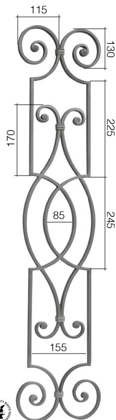
Art. GD173/1 □ 14 x 8 mm L 230 mm H 1000 mm
