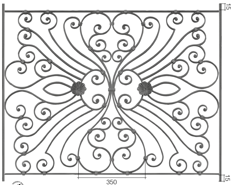
Art. GD239/1 □ 14 x 8 mm L 1185 mm H 1000 mm
