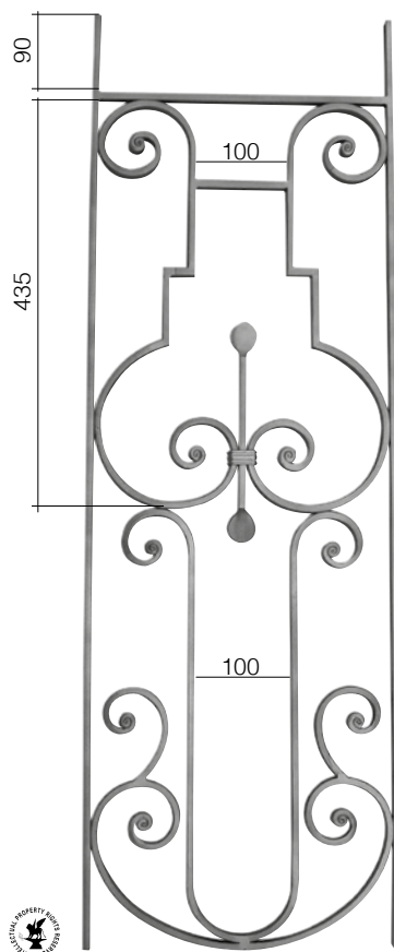
Art. GD245/1 □ 14 x 8 mm L 330 mm H 1000 mm
