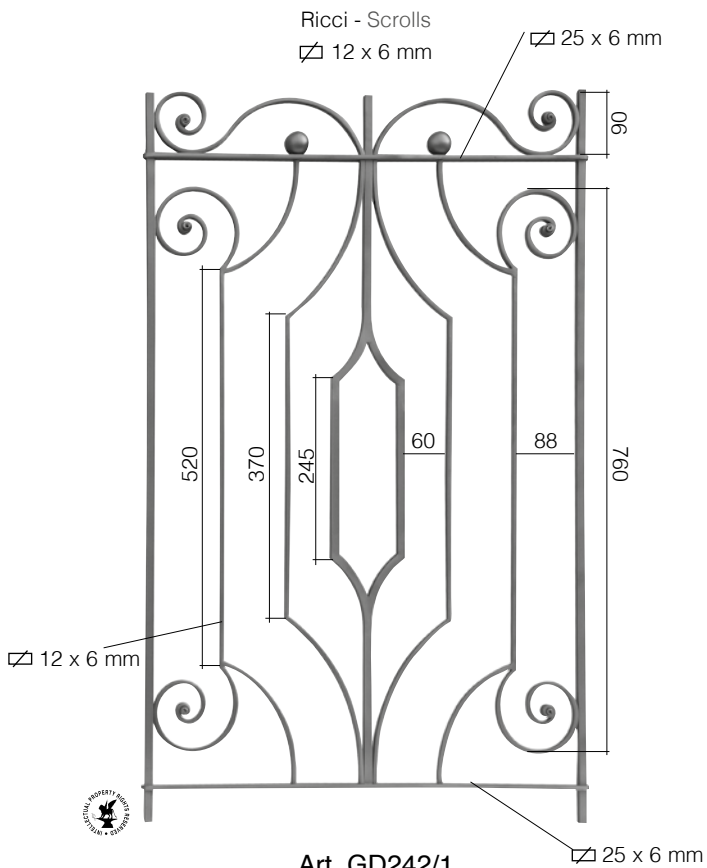
Art. GD242/1 ∅ 12 mm L 640 mm H 1000 mm
