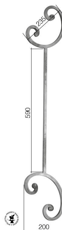
Art. GD22/5 ∅ 14 mm L 200 mm H 1000 mm
