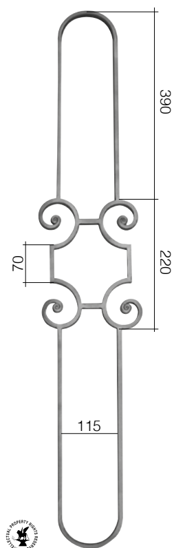
Art. GD245/3 □ 14 x 8 mm L 180 mm H 1000 mm
