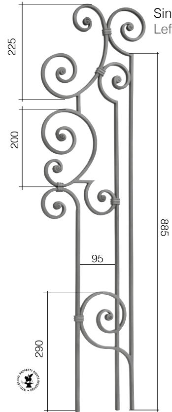
sinistro - left Art. GD163/2 □ 14 x 8 mm L 280 mm H 1000 mm
