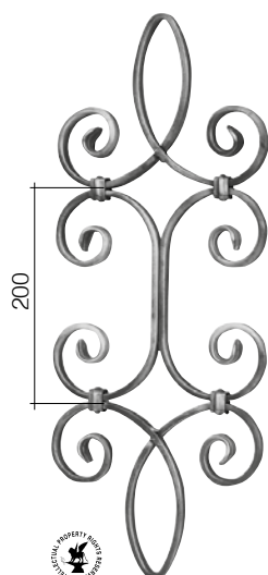
Art. 1647/2 □ 12 x 6 mm L 200 mm H 500 mm
