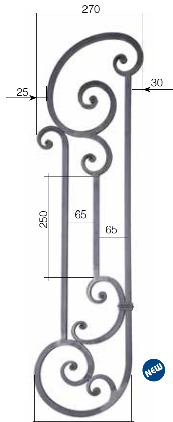
240 Art. GD32/2 ∅ 14 mm L 270 mm H 950 mm
