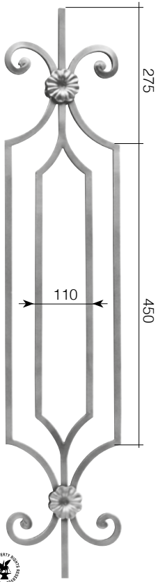
Art. 1685/3 Ø 14 mm L 230 mm H 1000 mm
