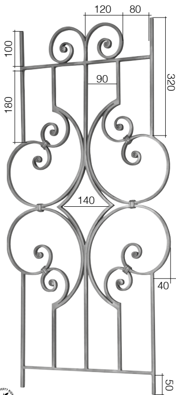
Art. GD219/1 □ 14 x 8 mm L 500 mm H 1000 mm
