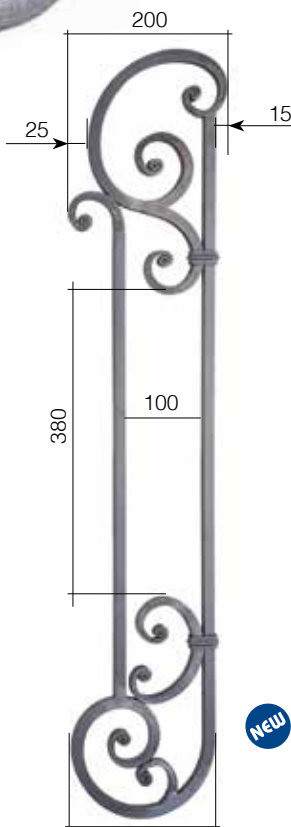
185 Art. GD32/1 ∅ 14 mm L 200 mm H 950 mm
