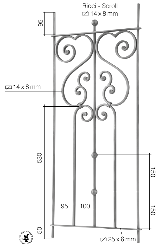
Art. GD241/1 Ø 12 mm L 450 mm H 1000 mm
