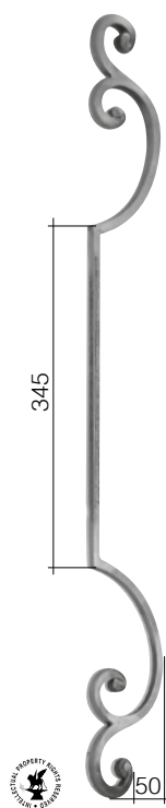
Art. GD22/3 ∅ 14 mm L 110 mm H 1000 mm
