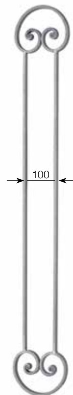
NEW Art. GD280/4 □ 14 x 8 mm L 155 mm H 1000 mm
