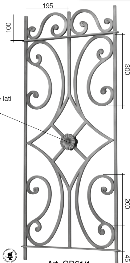
Art. GD61/1 □ 12 mm L 430 mm H 1000 mm
