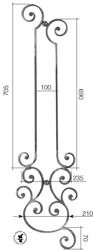
Art. GD159/2 □ 14 x 8 mm L 280 mm H 1000 mm
