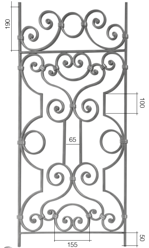
Art. GD216/3 □ 14 x 8 mm L 475 mm H 1000 mm
