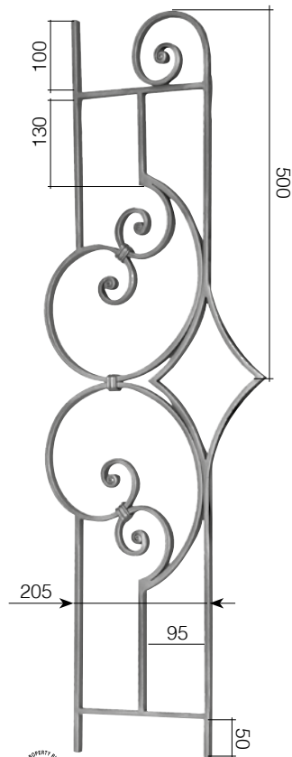
Art. GD219/2 □ 14 x 8 mm L 330 mm H 1000 mm
