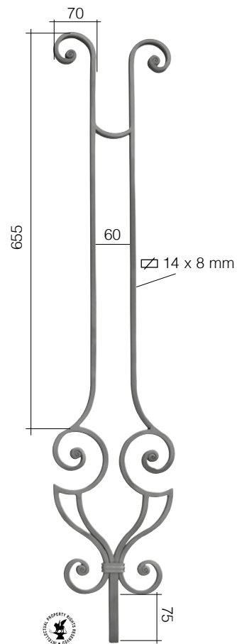
Art. GD148/1 \varnothing 14 mm L 205 mm H 1000 mm
