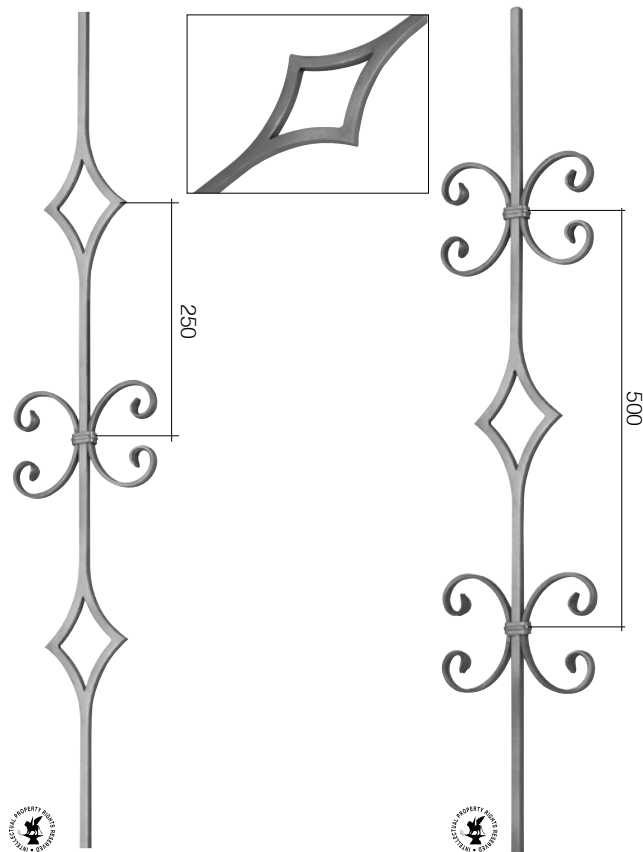
Art. GD59/3 \varnothing 12 mm L 200 mm H 1000 mm
