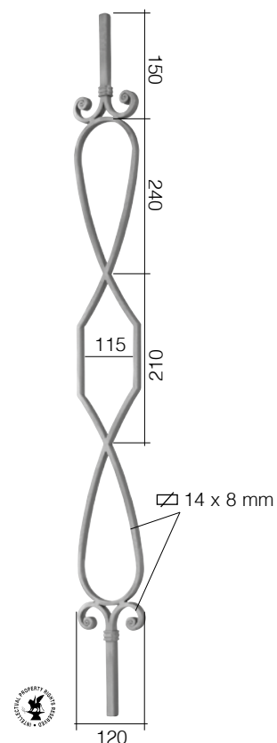
Art. GD178/1 □ 14 mm L 120 mm H 1000 mm
