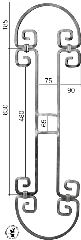
Art. 1142/2 \varnothing 12 mm L 280 mm H 1000 mm
