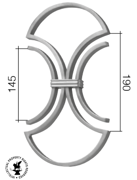
Art. GD187/2 \square 14 x 8 mm H 325 mm L 190 mm
