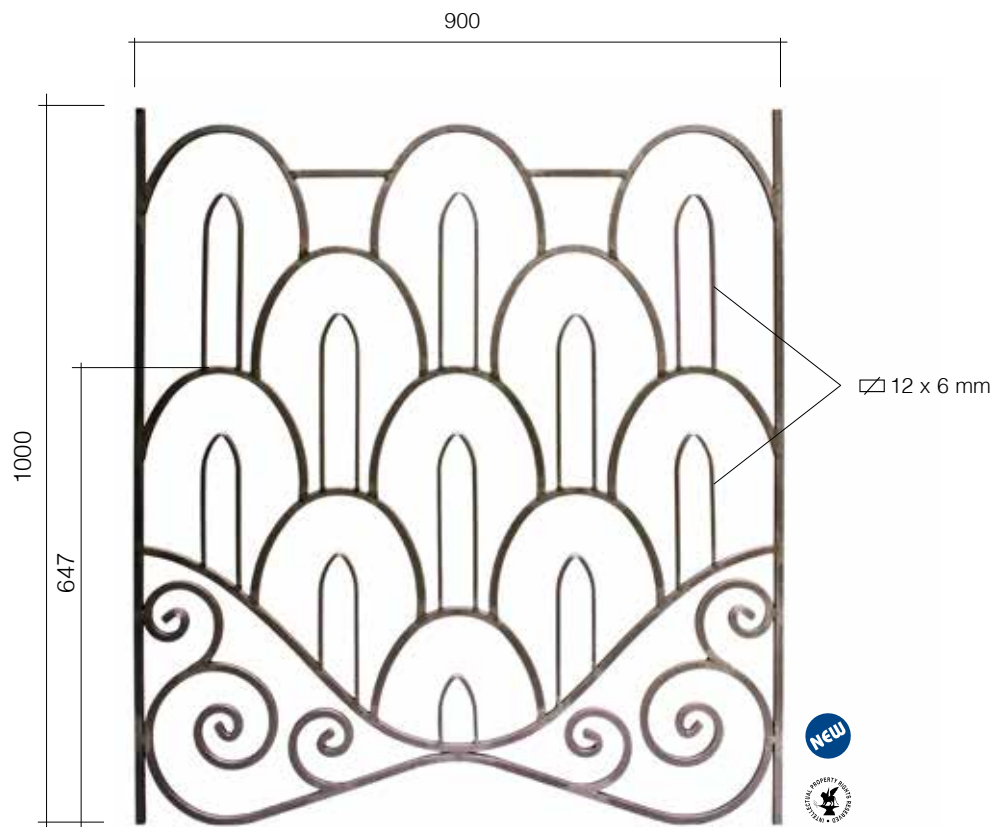
Art. GD291/1 Φ 12 x 12 mm + □ 12 x 6 mm L 900 mm H 1000 mm
