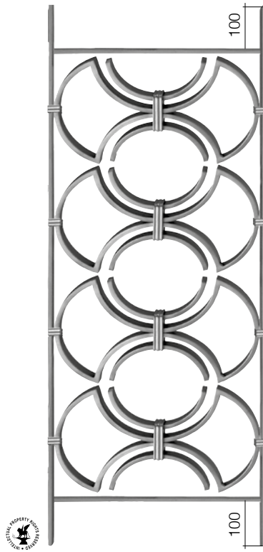
Art. GD189/2 \square 14 x 8 mm H 1000 mm L 340 mm
