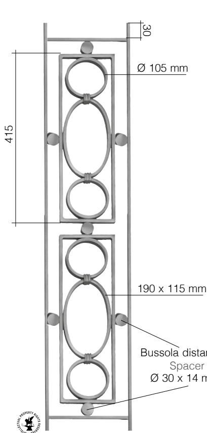
Art. GD205/2 \square 14 x 8 mm L 210 mm H 1000 mm
