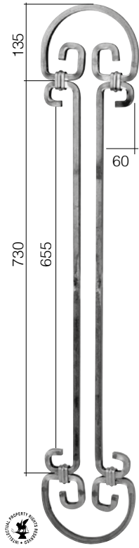
Art. 1142/1 \varnothing 12 mm L 180 mm H 1000 mm
