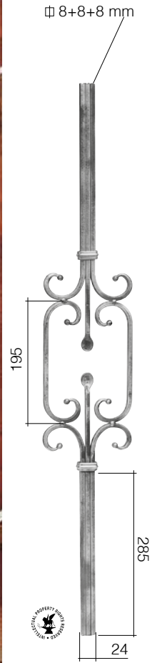
Art. 468/4 \varnothing 8 mm L 145 mm H 900 mm
