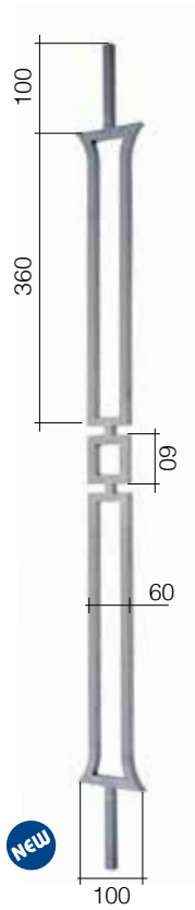
Art. GD78/4 \varnothing 12 mm L 100 mm H 1000 mm
