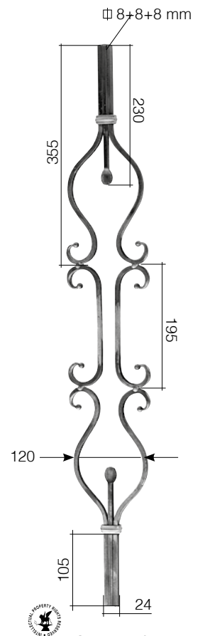
Art. 469/1 \varnothing 8 mm L 145 mm H 900 mm
