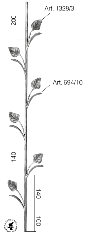
Art. 1170/1 Ø 12 mm L 130 mm H 1000 mm
