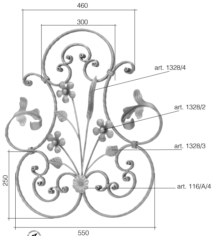
Art. GD269/1 □ 16 x 8 mm spigolato hammered on the edges 640 x 710 mm
