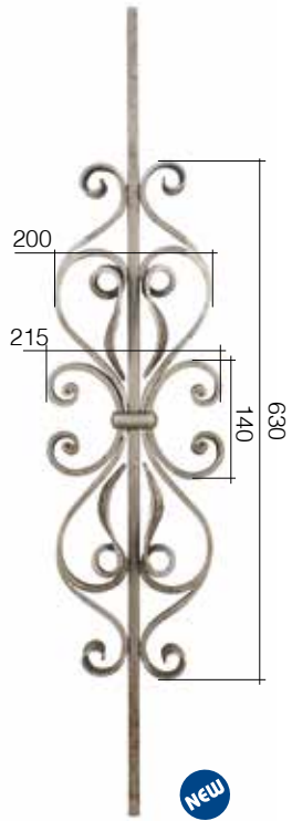
Art. GD28/1 \varnothing 14 mm L 215 mm H 1000 mm
