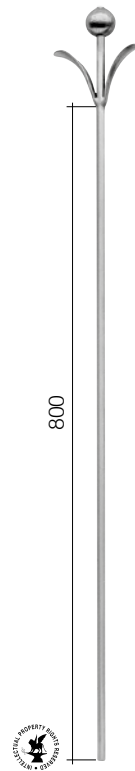
Art. 1170/3 Ø 12 mm L 130 mm H 1000 mm
