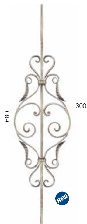
Art. GD27/1 \varnothing 14 mm L 300 mm H 1000 mm
