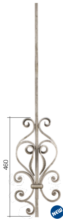
Art. GD28/3 \varnothing 14 mm L 215 mm H 1000 mm
