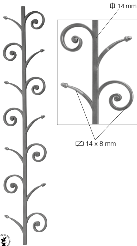
Art. GD176/1 \varnothing 14 mm L 200 mm H 1000 mm
