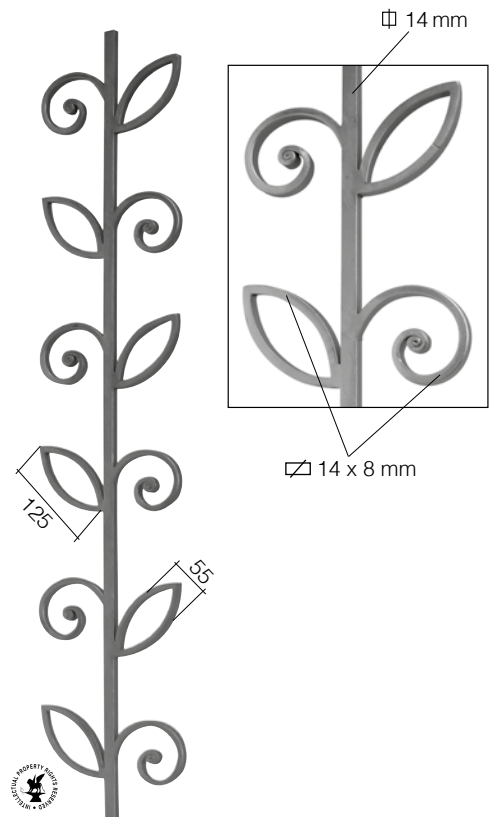
Art. GD176/3 \varnothing 14 mm L 200 mm H 1000 mm
