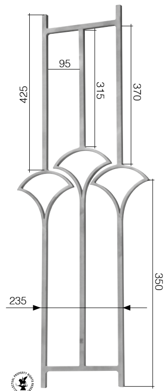
Art. GD186/3 \varnothing 14 mm L 390 mm H 1000 mm
