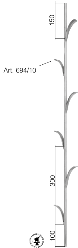
Art. GD92/2 Ø 12 mm L 130 mm H 1000 mm
