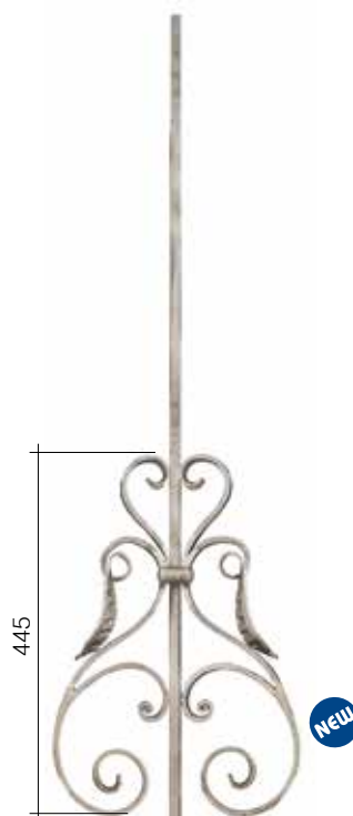
Art. GD27/2 \varnothing 14 mm L 300 mm H 1000 mm
