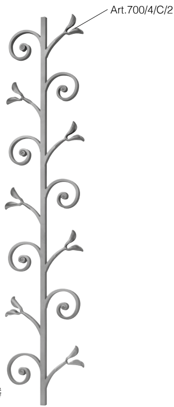
Art. 700/4/C/2 \varnothing 14 mm L 200 mm H 1000 mm
