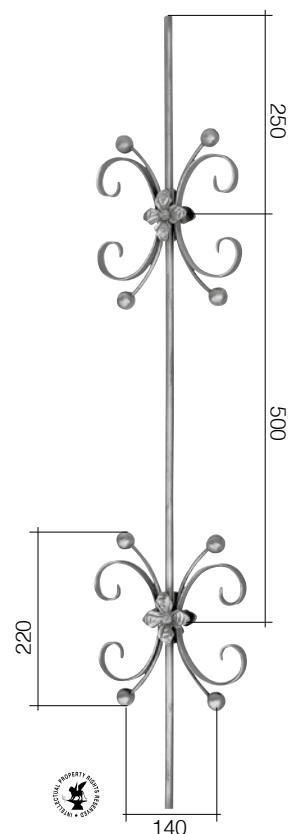
Art. 1061/2 Ø 12 mm H 1000 mm L 205 mm
